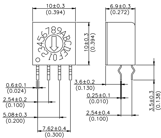
ERD4XXXR Flat Type
