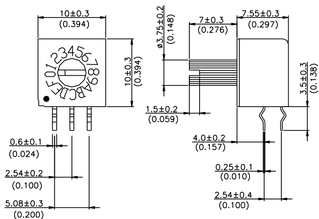
ERD2XXR Shaft Type
