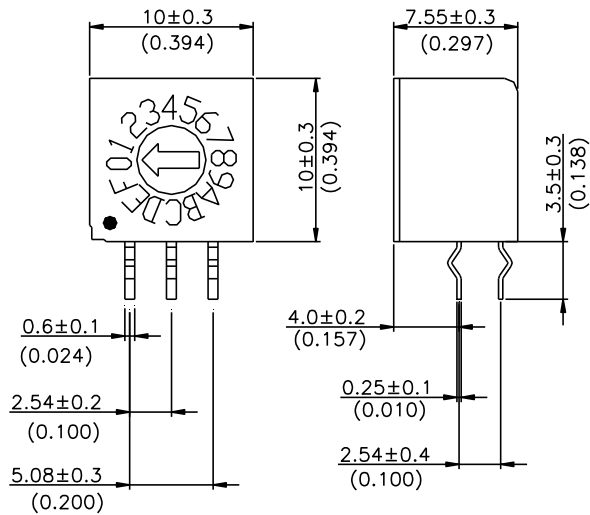
ERD1XXR Flat Type
