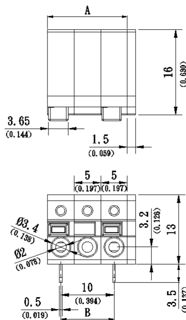
ETBH50xx1 Pitch=10.0mm
