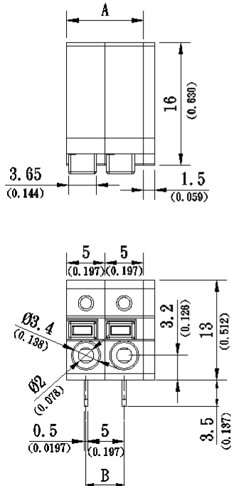
ETBH50xx0 Pitch=5.0mm
