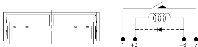
Wiring diagram (Top View)
