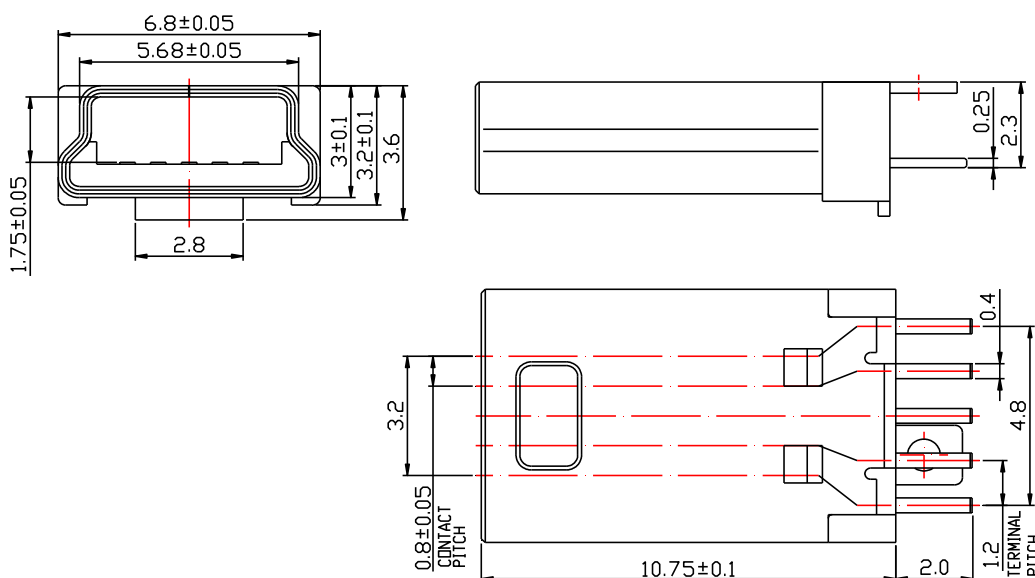
ESB3A B Type Plug (for 5 pin)
