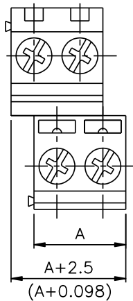
ETB18** Pitch=5.0mm
