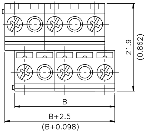
ETB18**1 Pitch=10.0mm
