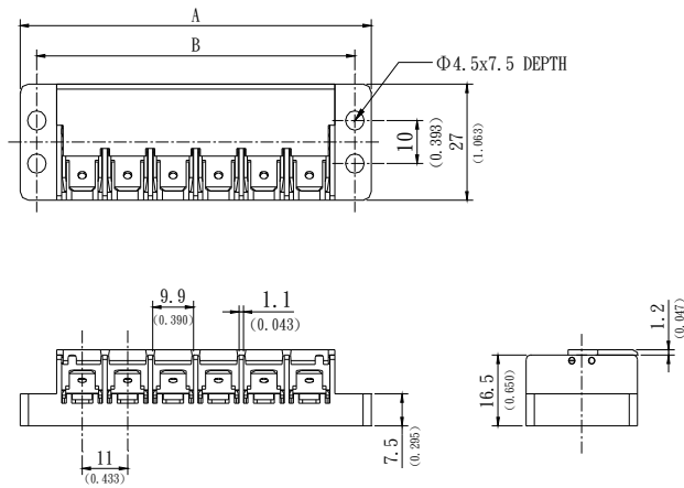
ETBT140X2F000Z #250 Quick connect terminal Pitch=11.0mm
